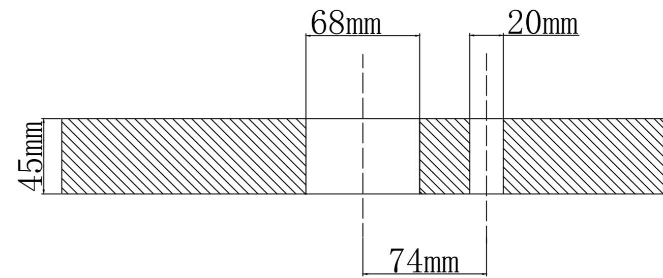
VIEW B-B
