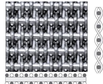
Reverse Plain Dutch Weave
