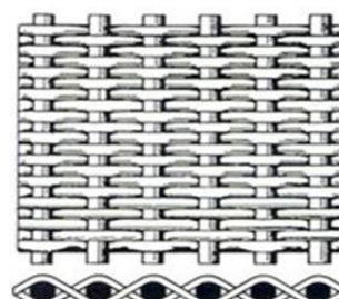
Plain Dutch Weave
