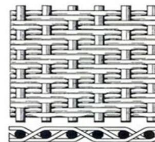
Twilled Dutch Weave
